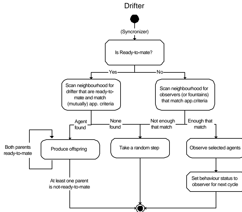
Figure 10 Agents with the status drifters, starts by scanning the neighbourhood for agents to observe or mate with, if none is found a random step is taken. Note that a drifter that mate keeps the drifter status for next cycle, as the next step after mating is finding someone to observe (do business with).
