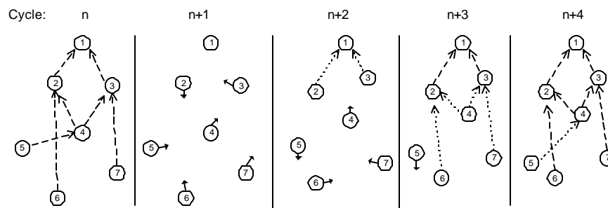
Figure 11 The behaviour of agents when connected to a single 'fix point' (agent 1) that starts drifting. (The dotted arrows illustrates that the agent will start observing in next cycle.)
