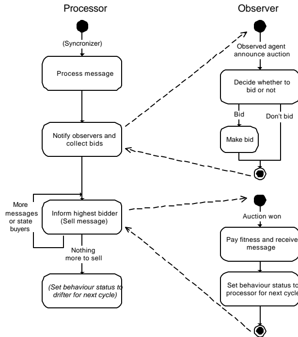
Figure 8 The processors activities are initiated by the main loop, whereas observers activities are synchronized by the processors.
