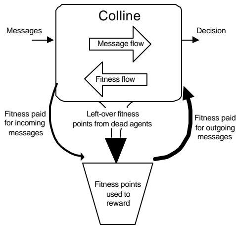
Figure 3 Two streams flows through Colline in opposite directions: The fitness flow and the message flow.
